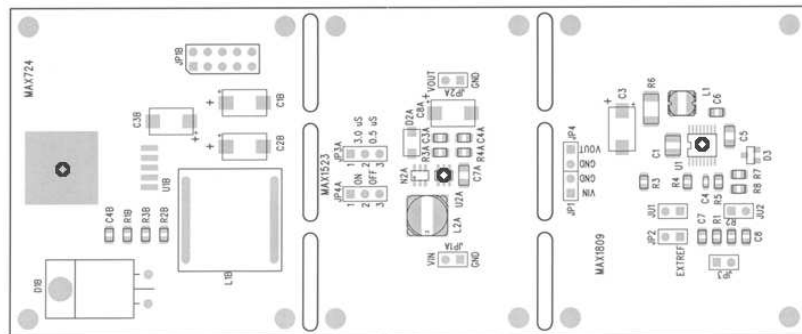
Fig. 7.20 - Custom board hosting the three MAXIM DC-DC converters; black circles indicates the DUTs.
