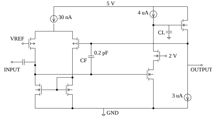
Fig. 3.9 - Design of the GTFE shaper; the signal from the preamplifier comes from the left through an input capacitance.
