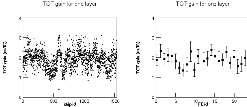
Fig. 8.6 - TOT gain for all 1536 channels in a TKR layer, and average values for the 24 GTFEs.
