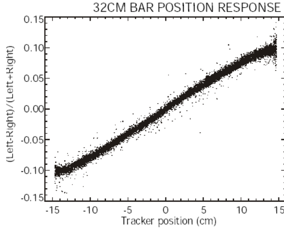
Fig. 3.5 - Left/right signal asymmetry in CAL crystals due to tapering for 2 GeV electrons ( \sim 130 \text{ MeV} deposited), from [45].
