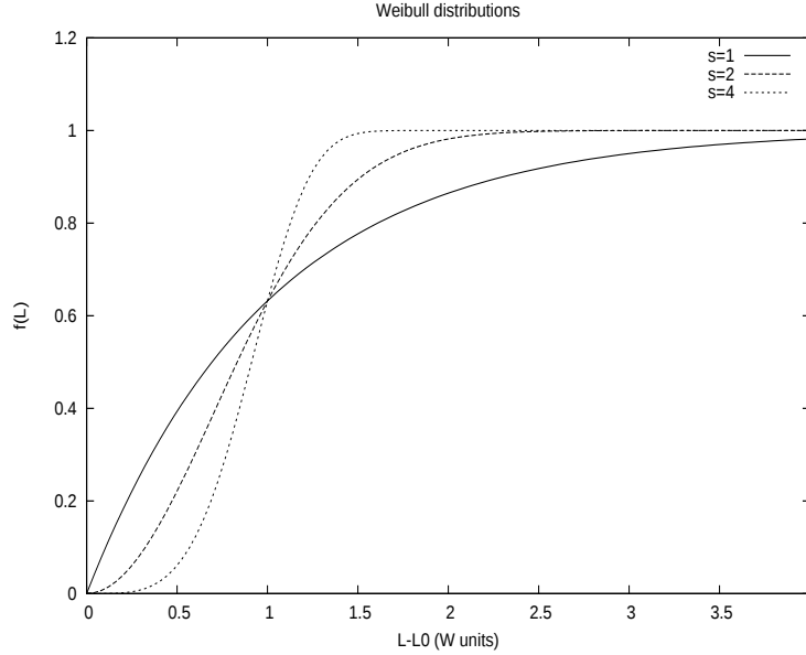
Fig. 5.4 - Weibull distribution functions for various shape parameters.
