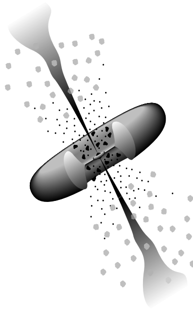
Fig. 1.2 - Artist rendition of an AGN: in the center the black hole, surrounded by the accretion disk, around it the warped torus.
