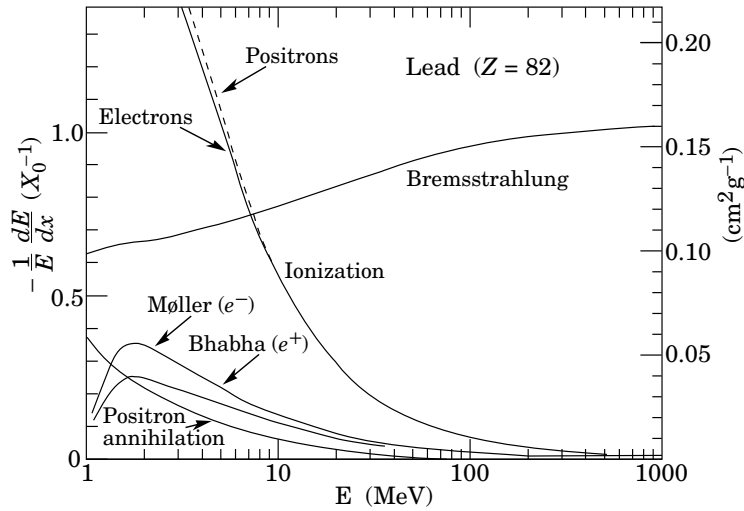
Fig. A1.4 - Fractional energy loss per radiation length in lead as a function of electron or positron energy [126].
