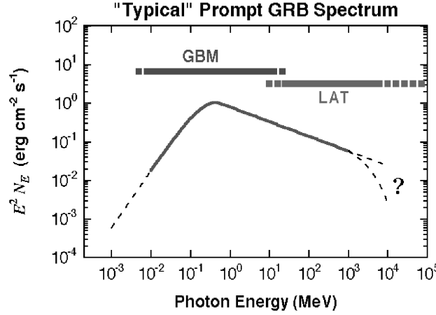
Fig. 1.7 - Energy coverage of GLAST LAT and GBM: the range of sensitivity of each instrument is shown on top of a sample GRB spectrum; a possible spectral break within the LAT range is shown.
