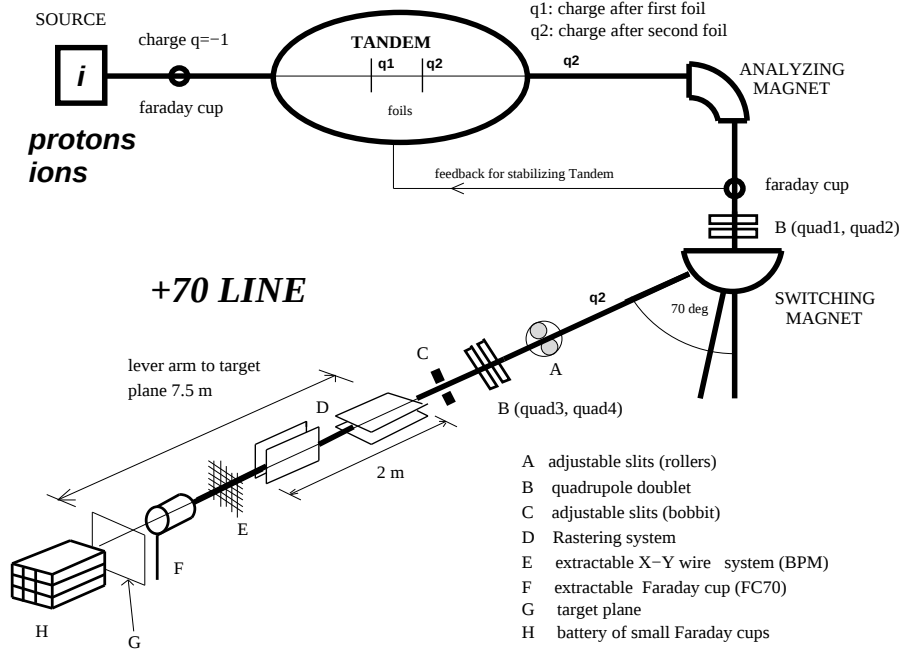
Fig. A3.2 - Schematics of the 15 MV Tandem-XTU at LNL and of the +70^\circ beam line where SIRAD is placed.
