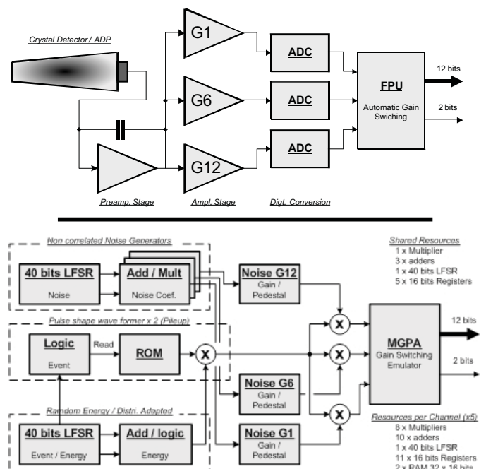
Figure 2: A schematic view of the VFE detector signal flow (top view) and the model used for XFEST (bottom view)
