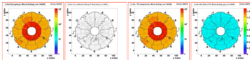
Figure 3.12: An example of distribution shown on the analysis page: a comparison between Level-1 isolated candidates, and their emulation from trigger primitives. From left to right: L1 isolated candidate occupancy; occupancy of L1 candidates for which no TP pairs were found; number of L1-TP comparisons; mean of the ratio \frac{L1}{TP_1+TP_2} for each region (turquoise corresponds to the expected value of 0.5).
